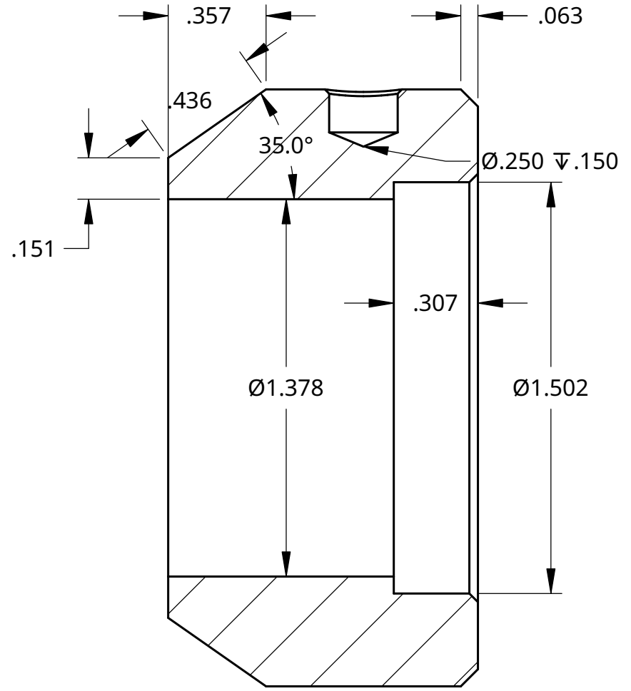
SECTION B - B SCALE 2:1
